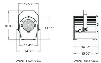
VN240 with barndoors
