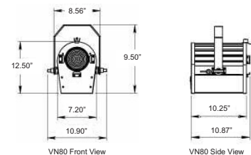
VN080 with C-clamp
