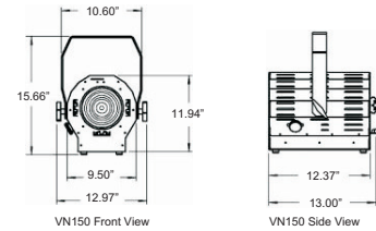
VN150 with barndoors
