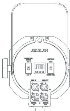
Pegasus 6" LED Fresnel Rear Controls. See manual.
