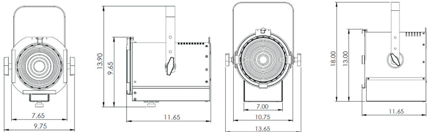
Pegasus 6" LED Fresnel Dim.
