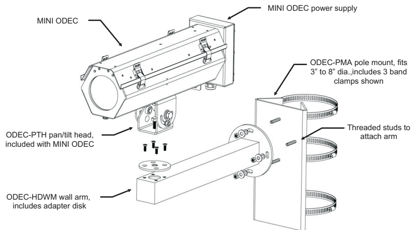
MINI ODEC with ODEC-PTH pan/tilt, ODEC-HDWM wall mount, and ODEC-PMA pole mount. Same mounting options for full size ODEC.
