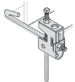
#ABC-1 Beam clamp with threaded rod
