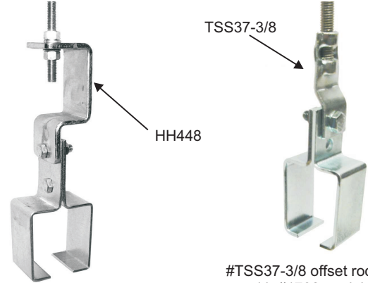
#HH448 bracket with 2808 track hanger
