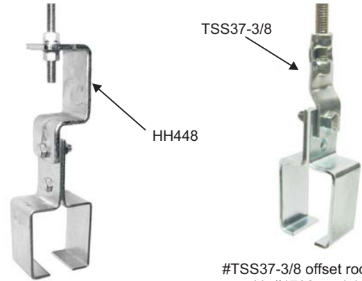
#HH448 bracket with 2808 track hanger
