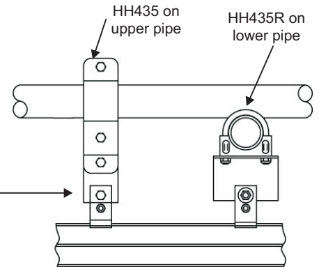
HH435 with HH435X and track hanger and HH435R with track hanger
