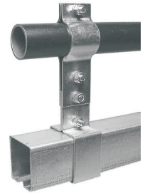
#2815 Batten Clamp with #2808 track hanger
